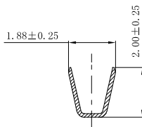
SECTION Y-Y
